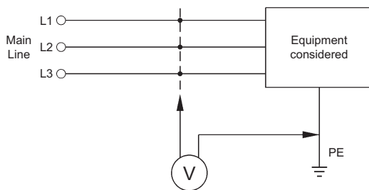
Fig. A: Common Mode Interference
